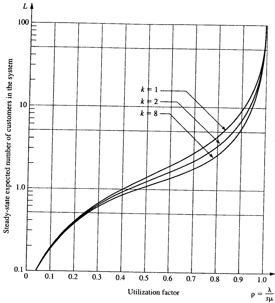
FIGURE 17.13 Values of L for the MIE_k/2 model (Sec. 17.7).
