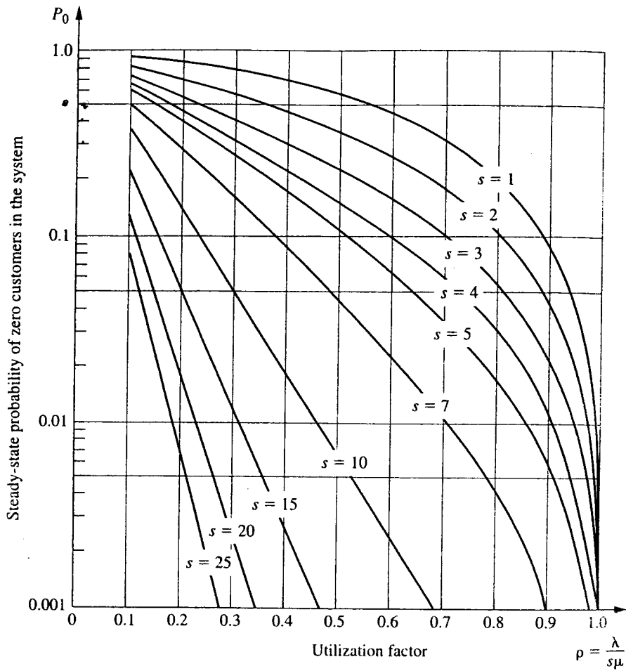
FIGURE 17.6 Values of P_0 for the MIM/s model (Sec. 17.6).
