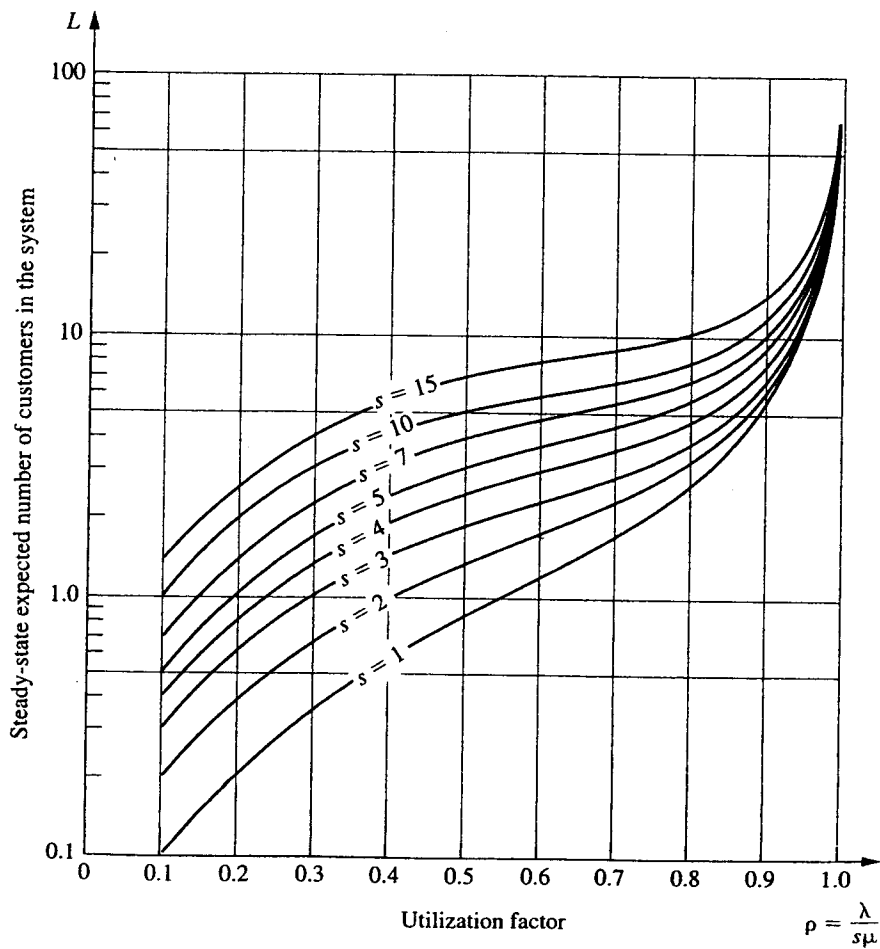
FIGURE 17.14 Values of L for the D/M/1/s model (Sec. 17.7).
