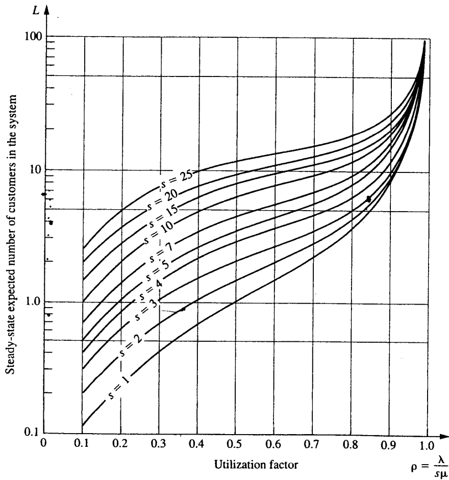
FIGURE 17.7 Values for L for the MIM/s model (Sec. 17.6).
